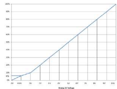
DIMMING GRAPH
