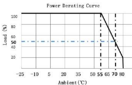
DERATING GRAPH
