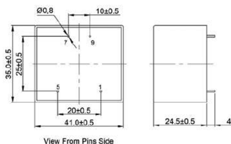
View From Pins Side
