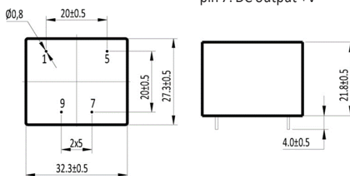
View From Pins Side
